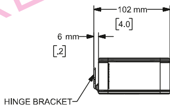
Left View
